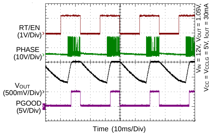
Pre-Bias Startup
