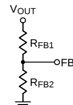
Figure 3. Output Voltage Setting
