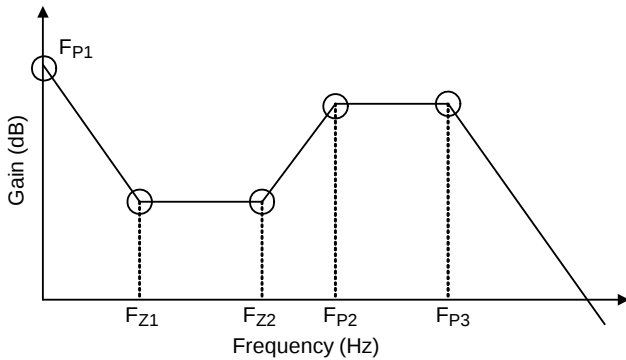
Figure 7. Bode Plot of the Type-III Compensation
