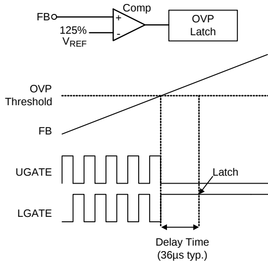
Figure 5. OVP Operation
