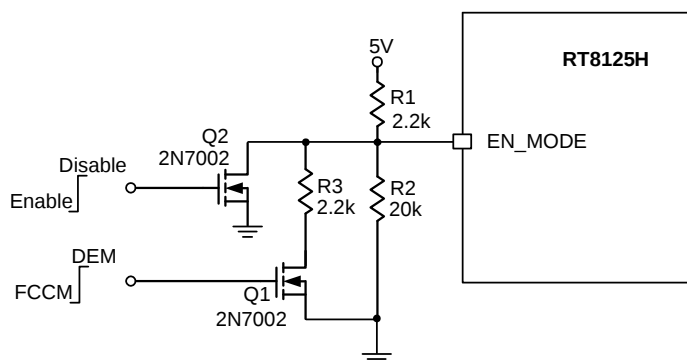
Figure 1. EN_MODE Pin Recommend Circuit
