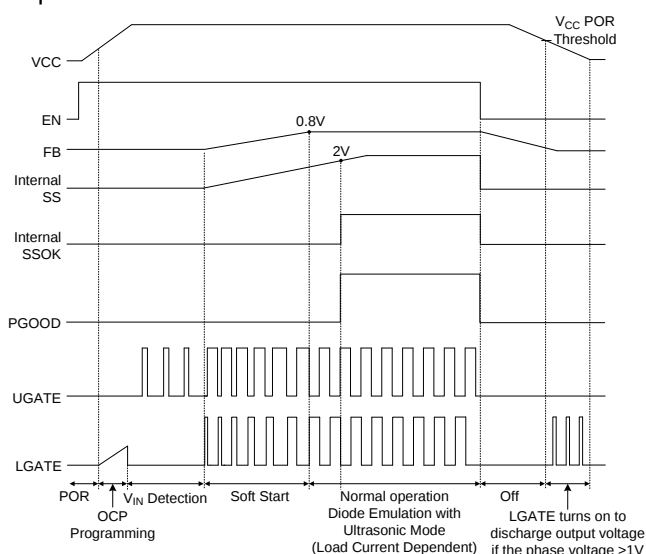
Figure 2. Soft-Start Sequence
