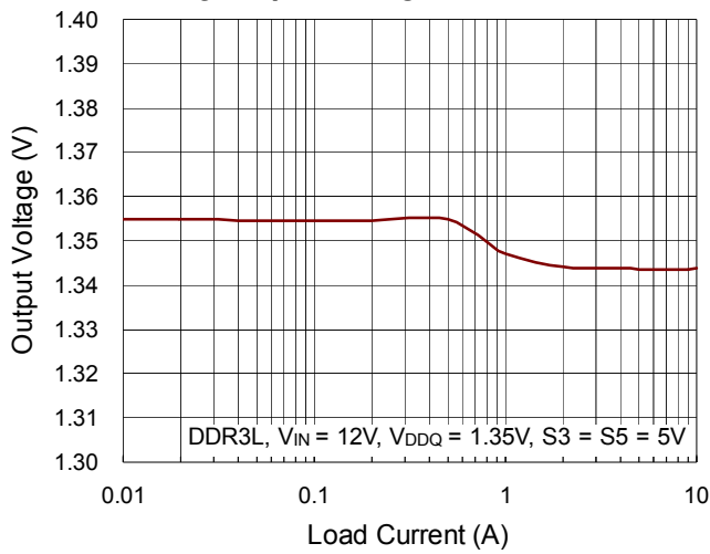
VDDQ Output Voltage vs. Load Current
