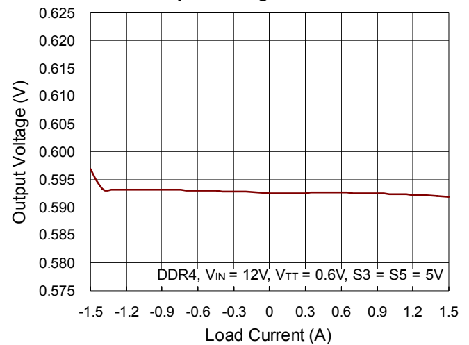
VTT Output Voltage vs. Load Current
