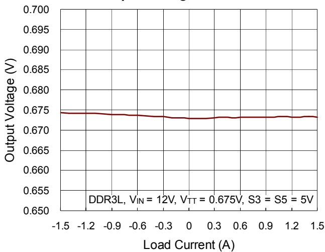
VTT Output Voltage vs. Load Current
