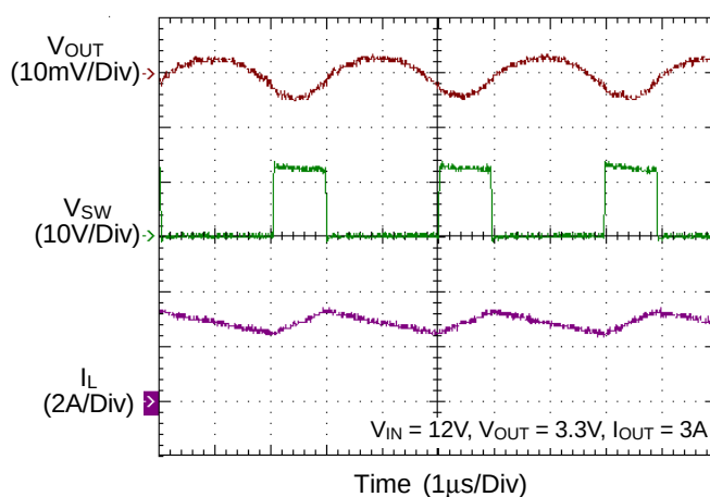
Switching Waveform
