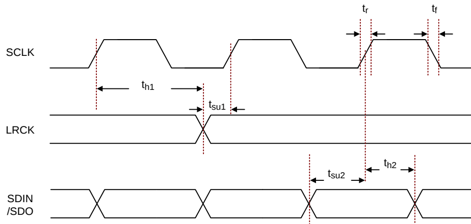
Figure 2. Timing Diagram of Slave Mode I²S Interface
