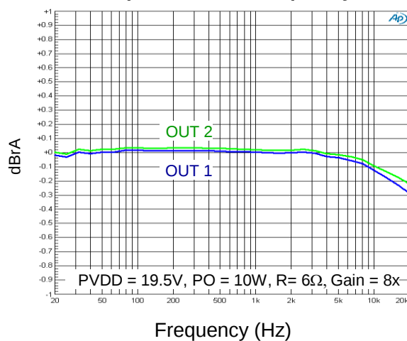
Output Level vs. Frequency
