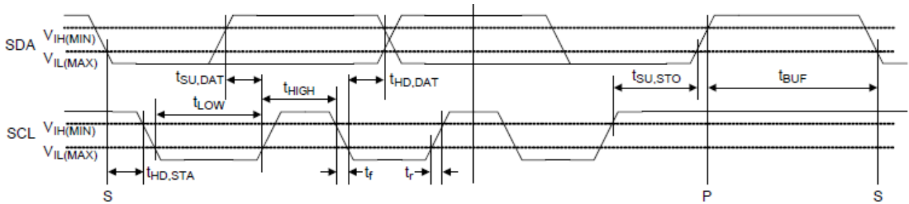
Figure 1. I²C Interface Trimming Diagram
