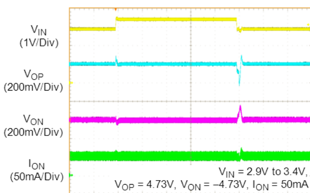
V ON Line Transient
