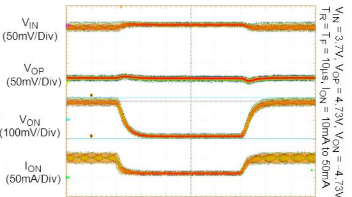
V ON Load Transient
