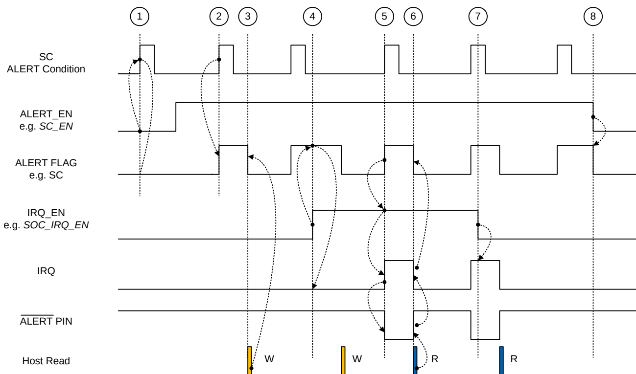
Figure 2. SC ALERT Function Timing Diagram
