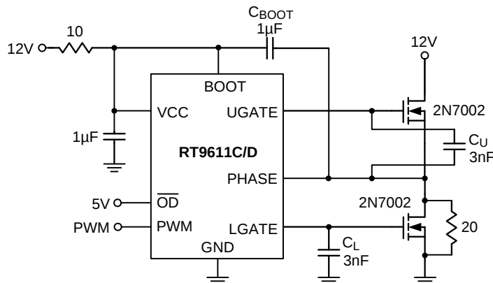
Figure 3. Test Circuit
