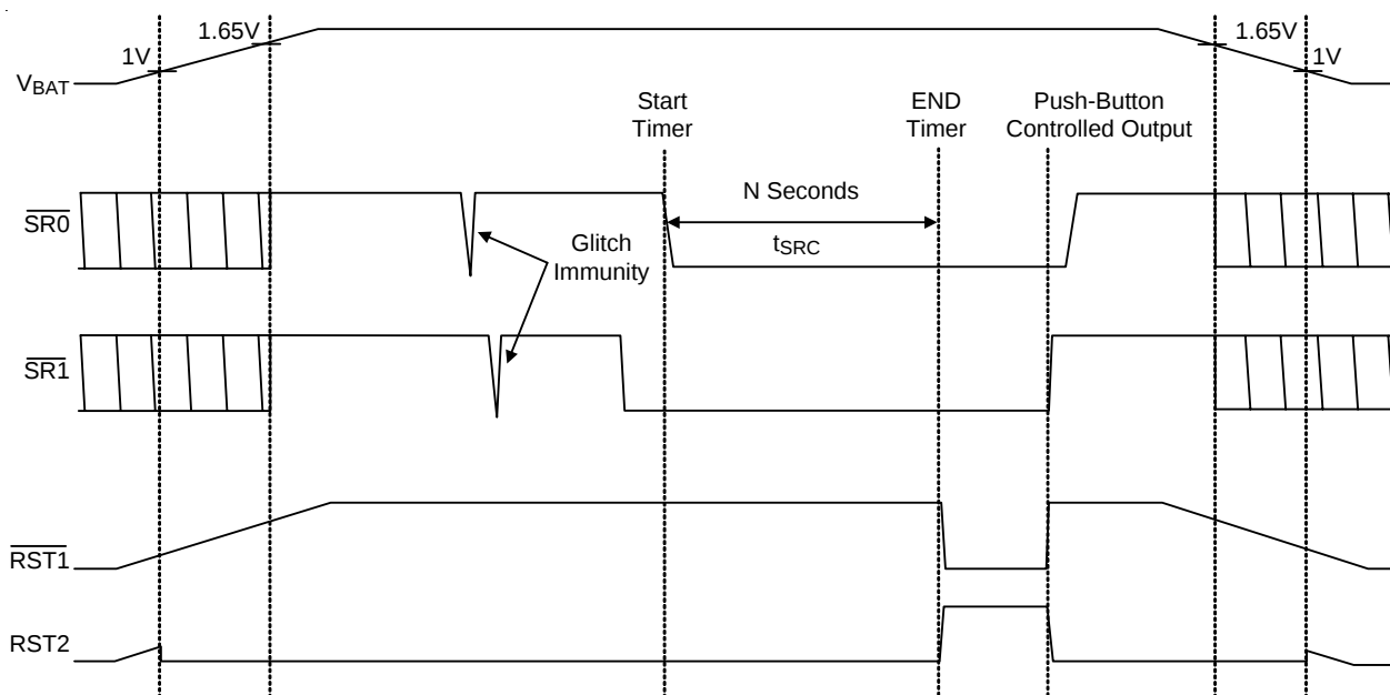
Figure 1. Timing Diagram
