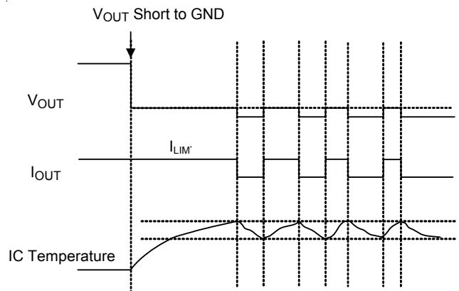
Figure 8. Short-Circuit Protection when Output Short-Circuit Occurs
