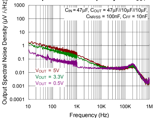
Output Noise vs. Frequency and V_{OUT}
