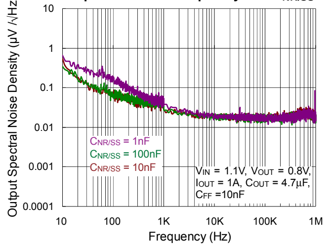
Output Noise vs. Frequency and C_{NR/SS}
