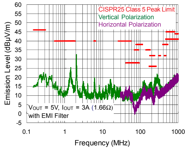
Radiated EMI Performance with Peak Limits
