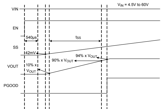
Figure 1 Start-Up Sequence for RTQ2965GQW
