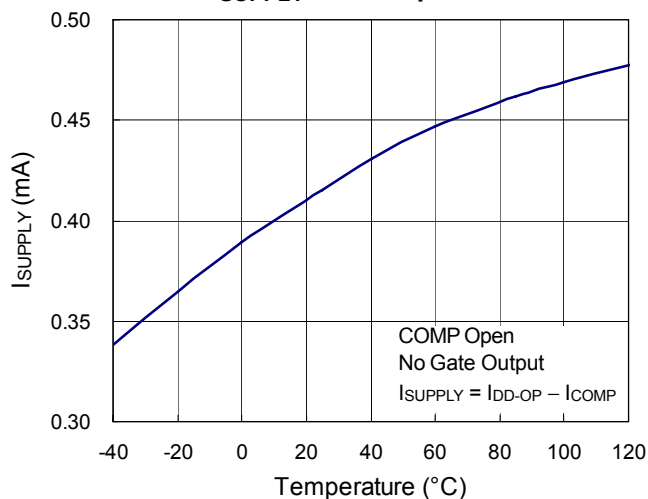
ISUPPLY vs. Temperature
