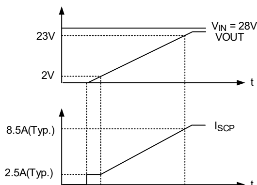
Figure 4. Short-Circuit Protection
