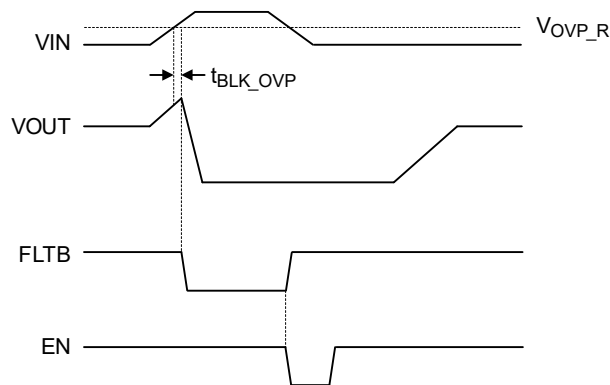
Figure 2. Overvoltage Protection
