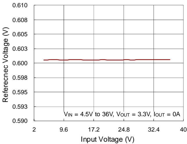
Referenc Voltage vs. Input Voltage
