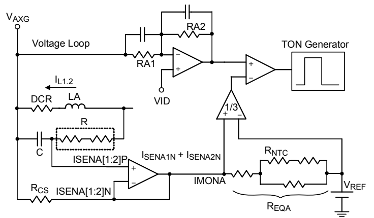
Figure 30. Voltage Loop and Current Loop
