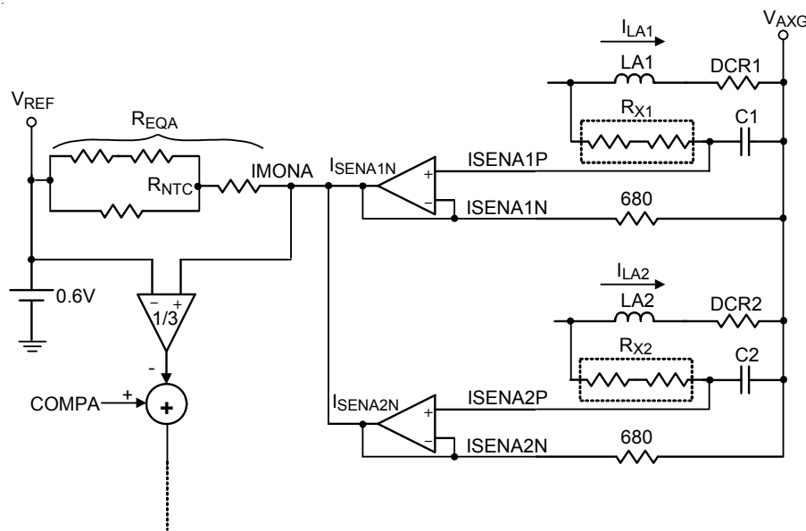
Figure 35. Current Loop Structure
