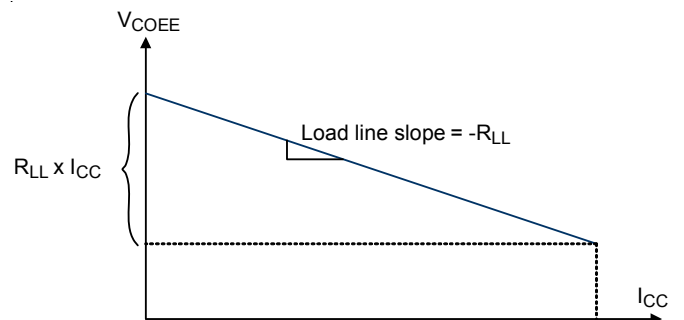
Figure 14. Load-Line (Droop)
