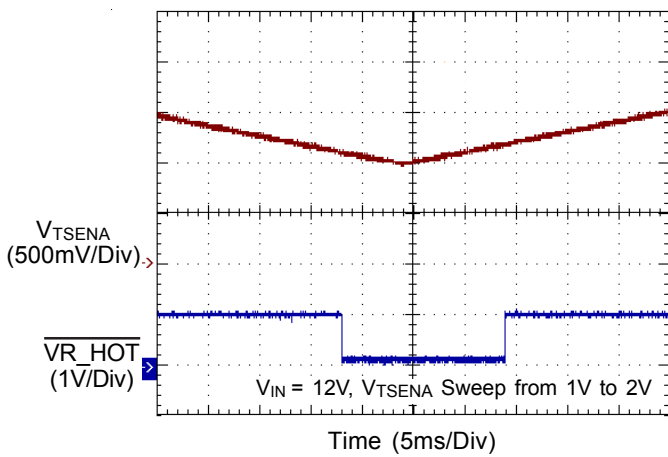
AXG VR Thermal Monitoring
