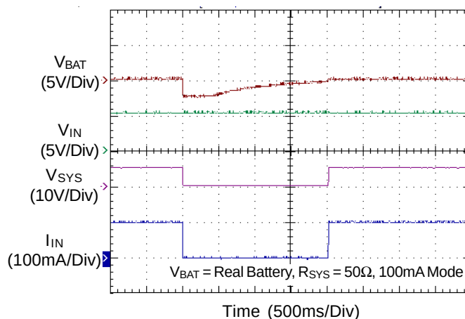
V_{IN} Exist then Negative Battery and Plug-out
