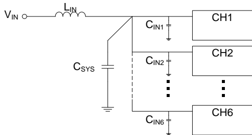
Figure 3. The Location of Bulk Input Capacitance Diagram
