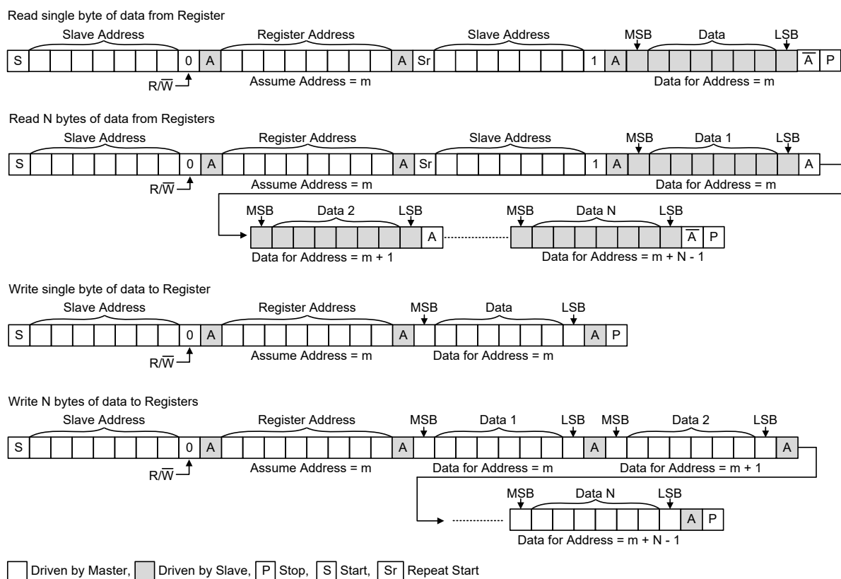
Figure 6. I 2 C Timing Diagrams
