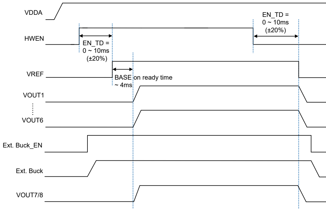
Figure 1. Power-ON/OFF Control
