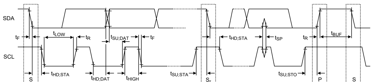
Figure 7. I 2 C Waveform Information
