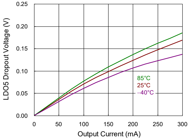
LDO5 Dropout Voltage vs. Output Current
