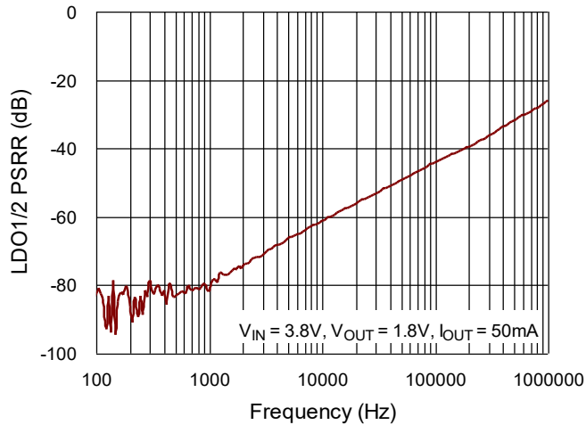
LDO1/2 PSRR
