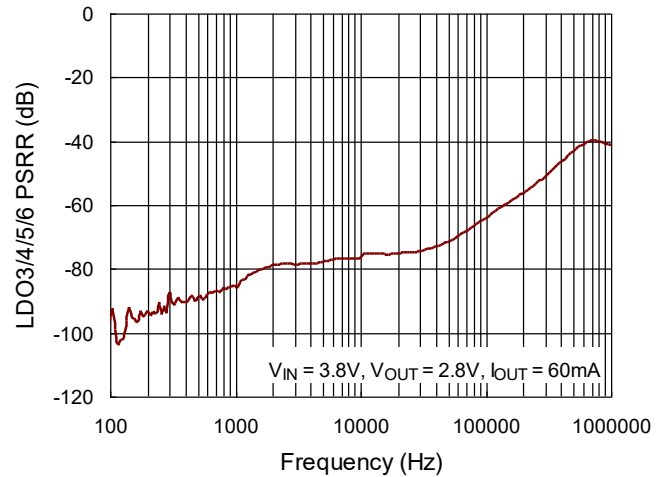
LDO3/4/5/6 PSRR
