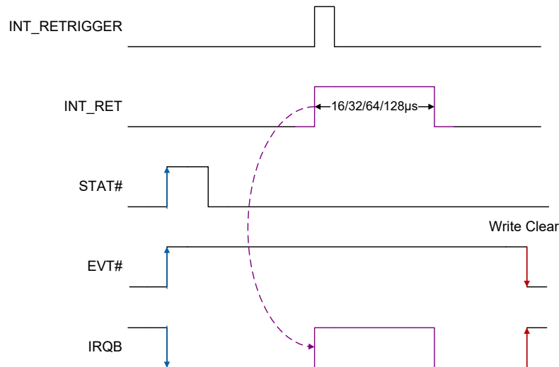
Figure 3. IRQB Pin Diagram
