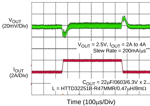
B1 Load Transient Response
