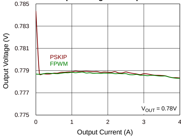
B3 Output Voltage vs. Output Current
