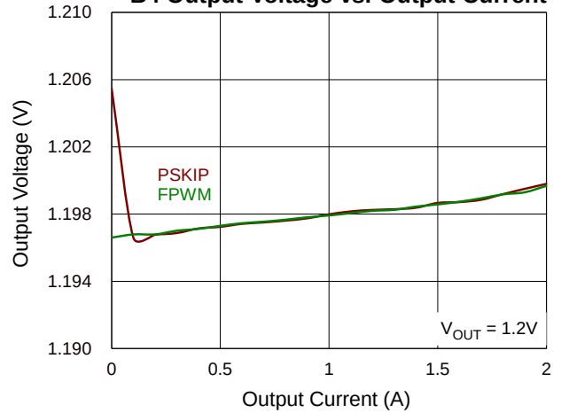
B4 Output Voltage vs. Output Current
