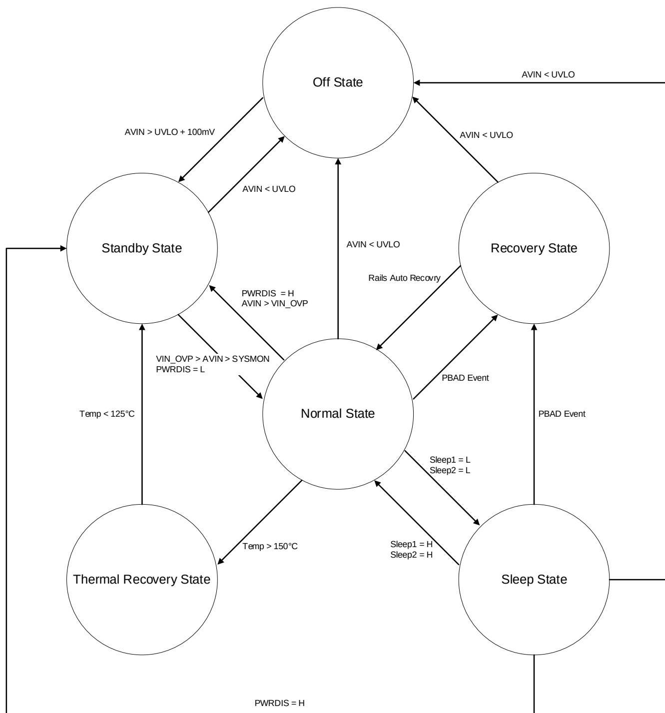
Figure 5. RT5147 State Machine
