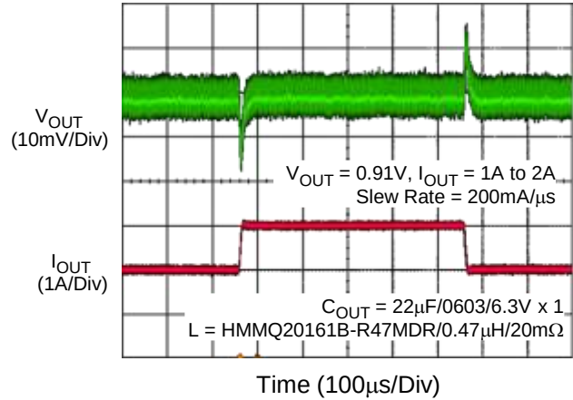
B2 Load Transient Response
