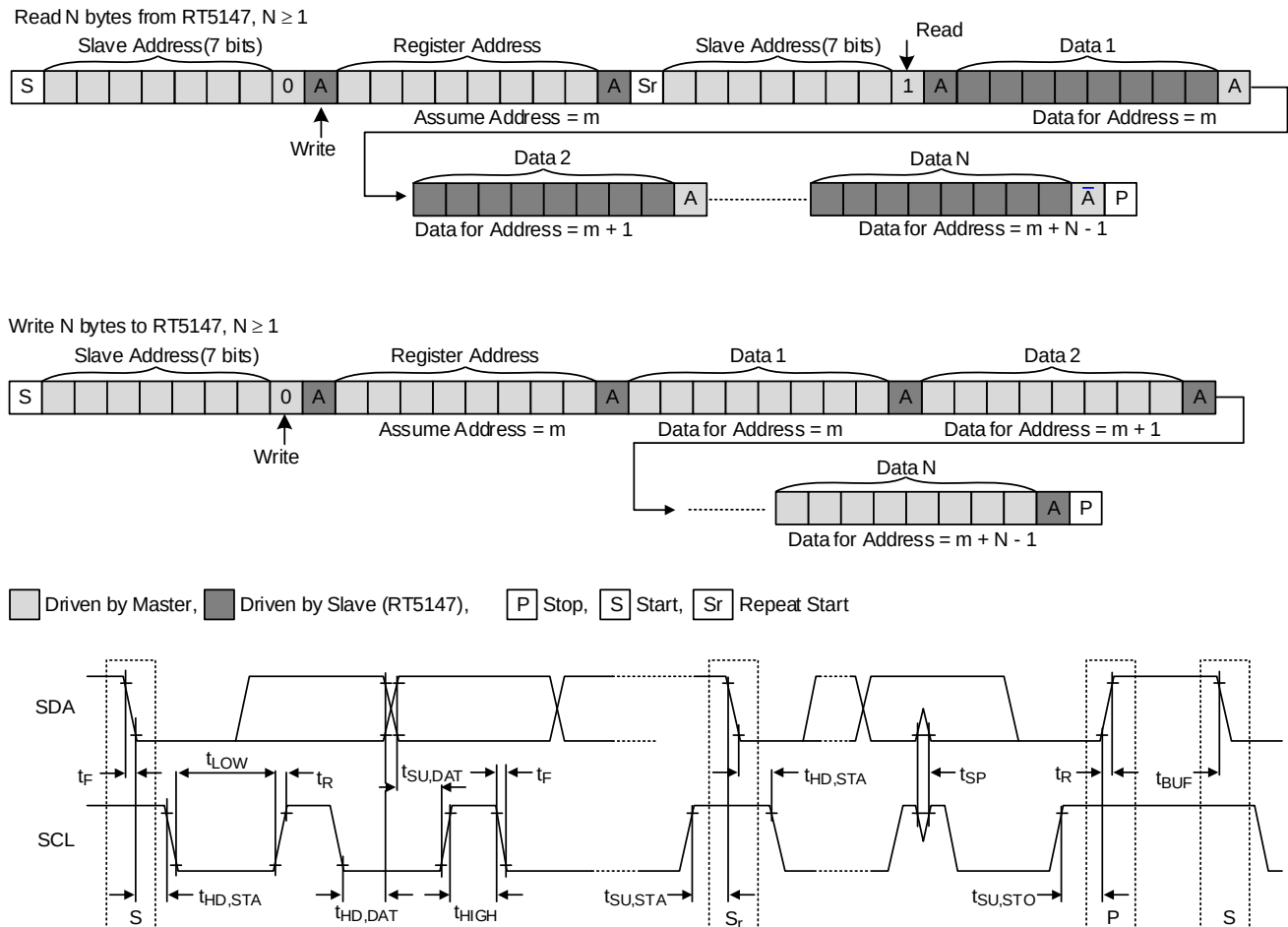
Figure 4. I 2 C Read/Write Stream and Timing Diagram
