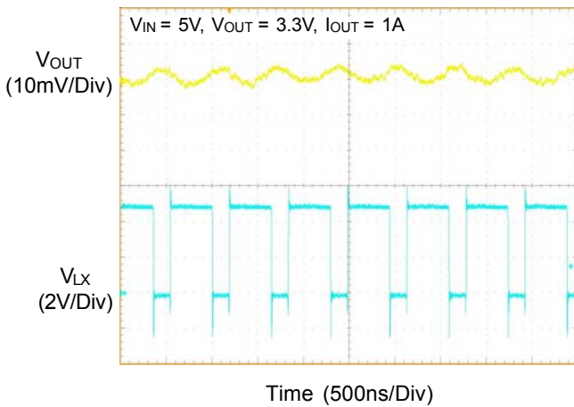
Voltage Ripple
