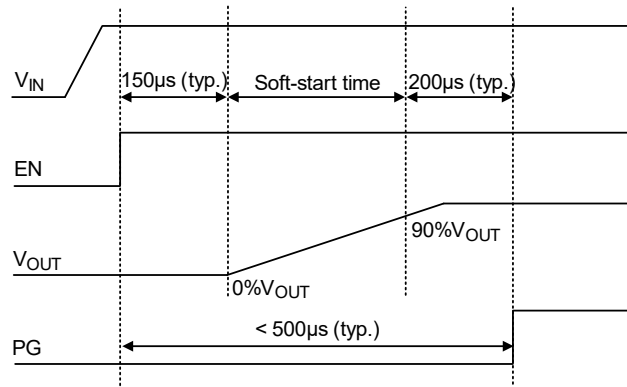
Figure 3. Start-Up Sequence without EN Delay
