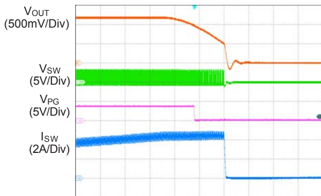
Figure 2. Overcurrent Protection
