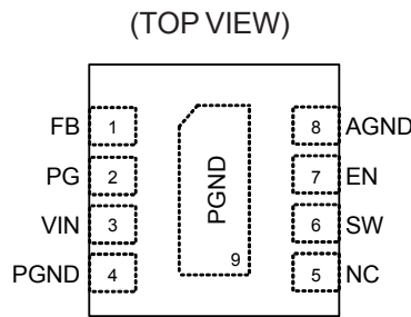
WDFN-8L 2x2/WDFN-8SL 2x2
