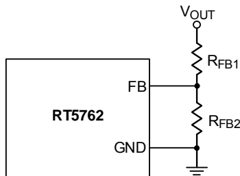
Figure 5. Output Voltage Setting
