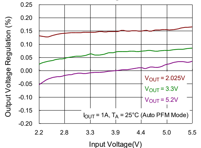
Line Regulation
