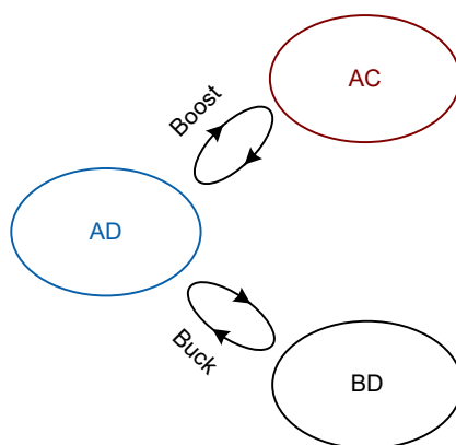
Figure 3. Buck-Boost Operation
