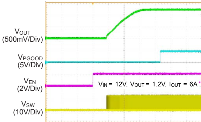
Time (2ms/Div)
