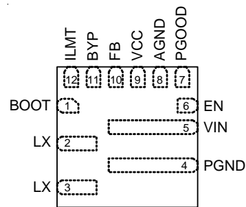
UQFN-12HL 3x3
