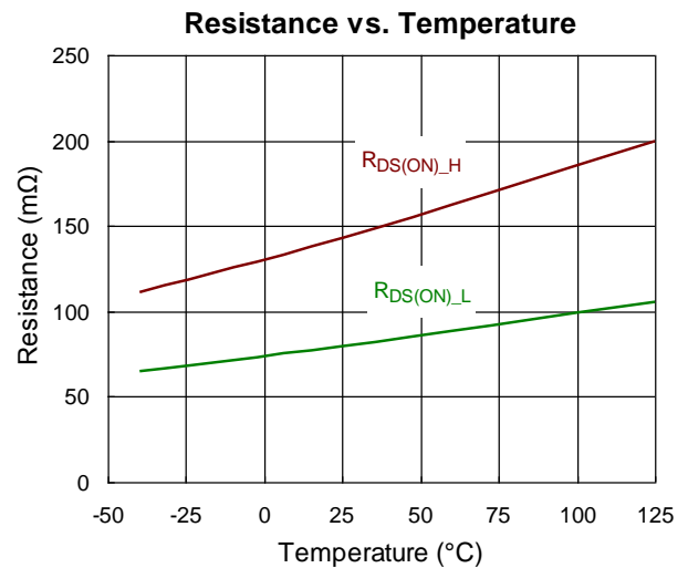
Figure 13. RT6352A/B R_{DS(ON)} vs. Temperature
