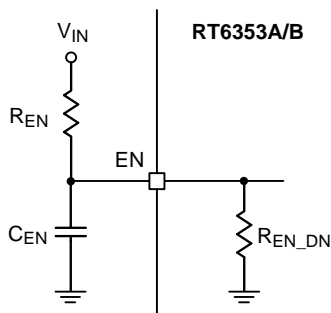
Figure 6. Automatic Start-Up Setting
