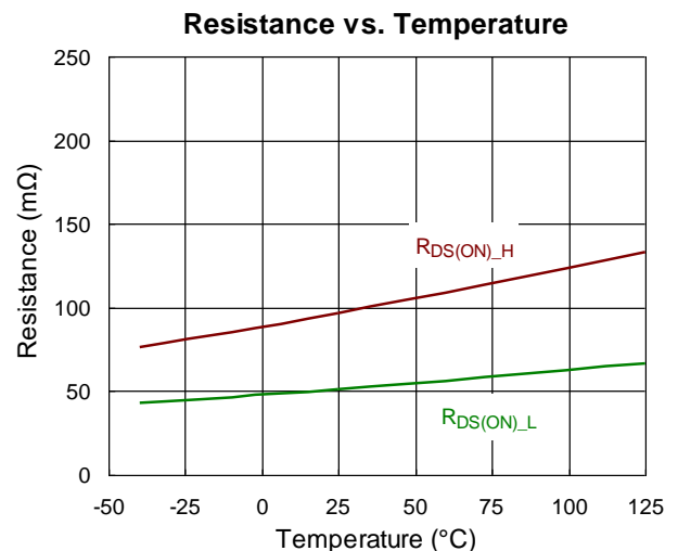
Figure 13. RT6353A/B R_{DS(ON)} vs. Temperature
