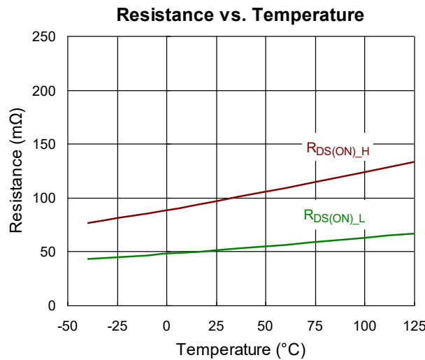
Figure 13. R_{DS(ON)} vs. Temperature
