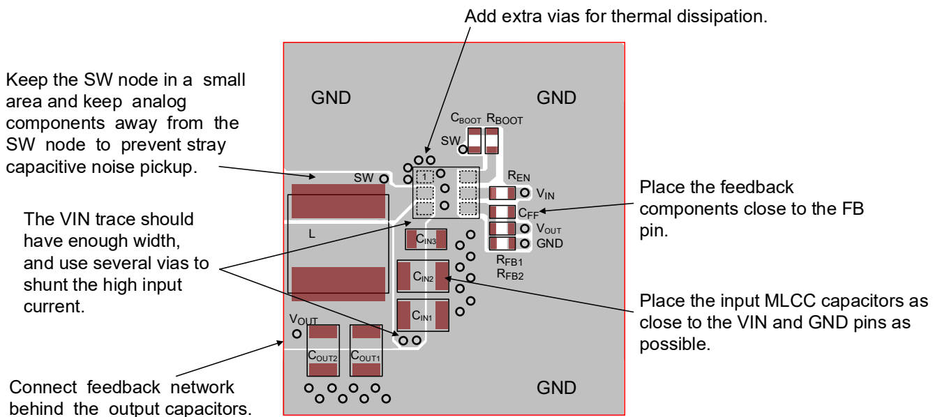
Figure 14. Layout Guide
