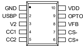
SOP-10 (RT7202KH)
