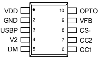
SOP-10 (RT7202KF/KP)
