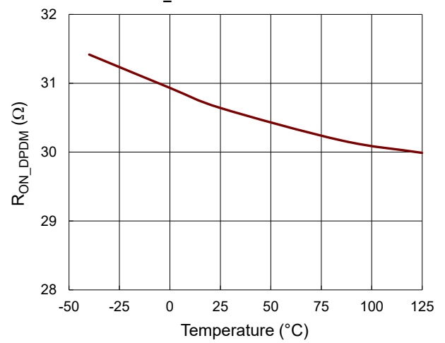
R_{ON\_DPDM} vs. Temperature
