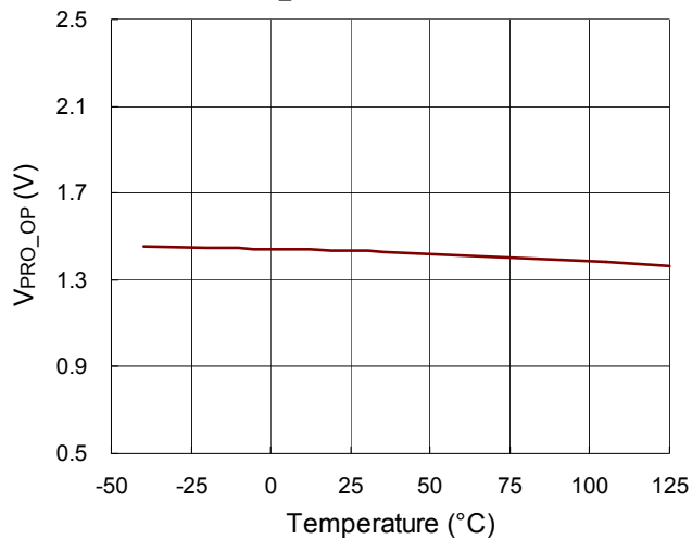
V PRO_OP vs. Temperature
