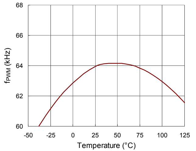
f PWM vs. Temperature
