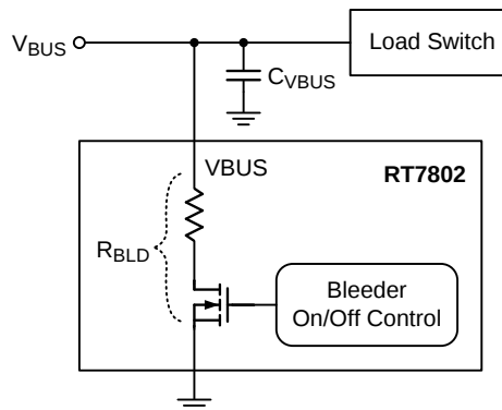
Figure 1. Bleeder Functional Block Diagram
