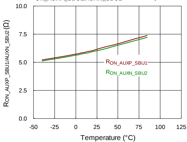
R_{ON\_AUXP\_SBU1/AUXN\_SBU2} vs. Temperature
