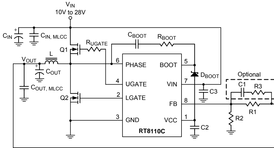
Figure 1. Typical Application Circuit for 10V to 28V Input Voltage
