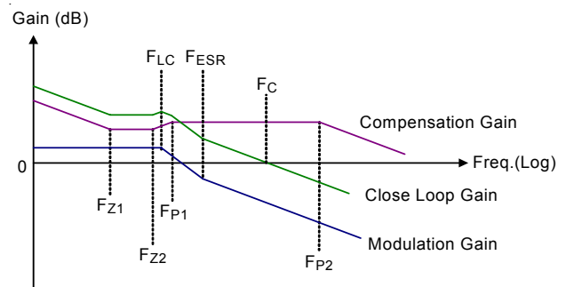
Figure 7. Bode Plot of Loop Gain.
