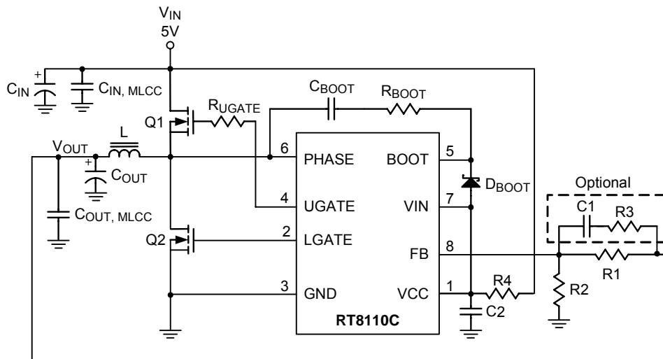
Figure 2. Typical Application Circuit for 5V Input Voltage
