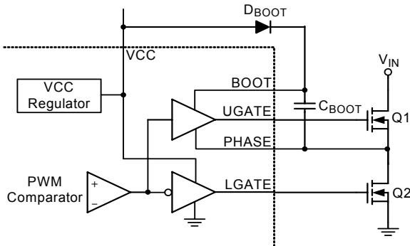
Figure 4. Gate Driver and Bootstrap Circuit
