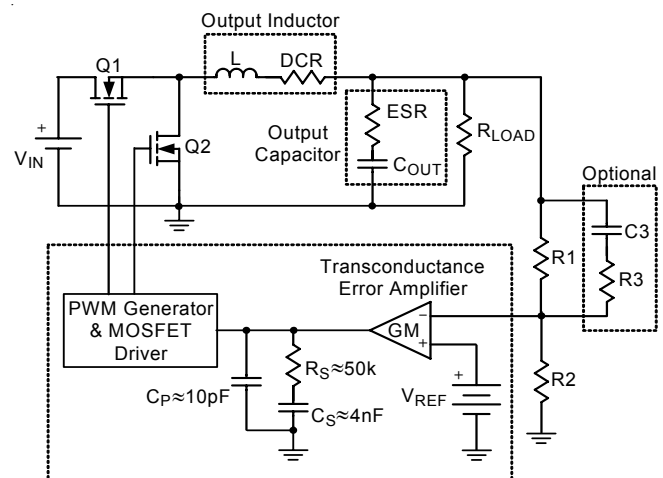
Figure 8. Simplified Diagram for Synchronous Buck Converter with Internal Compensation Network
