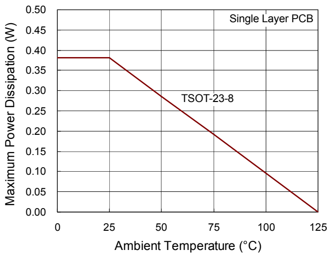
Figure 9. Derating Curves for RT8110C Package
