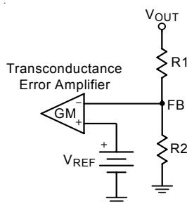
Figure 6. Voltage Divider Resistors
