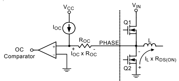
Figure 5. Over Current Protection Mechanism
