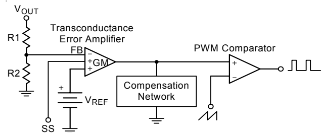
Figure 3. Transconductance Amplifier and PWM Comparator.
