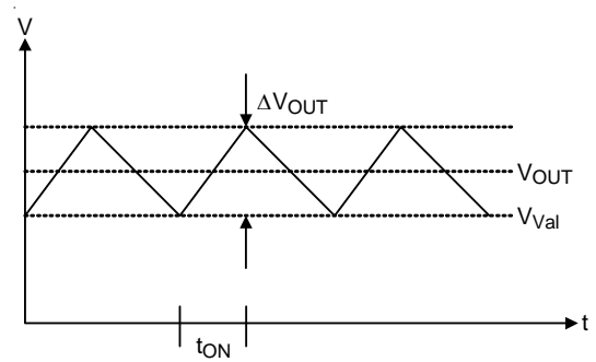
Figure 3. Output Voltage Waveform
