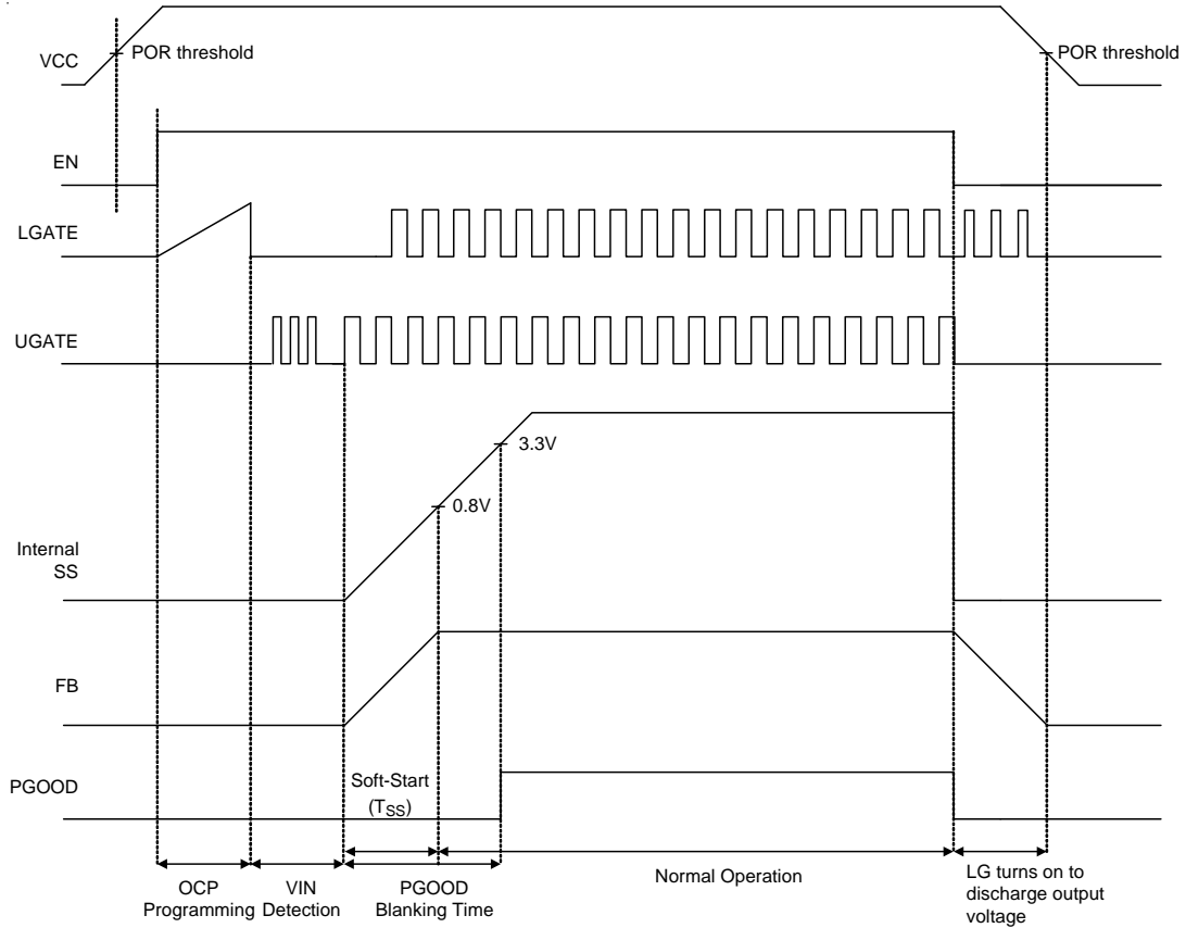
Figure 1. Soft-Start Timing Chart
