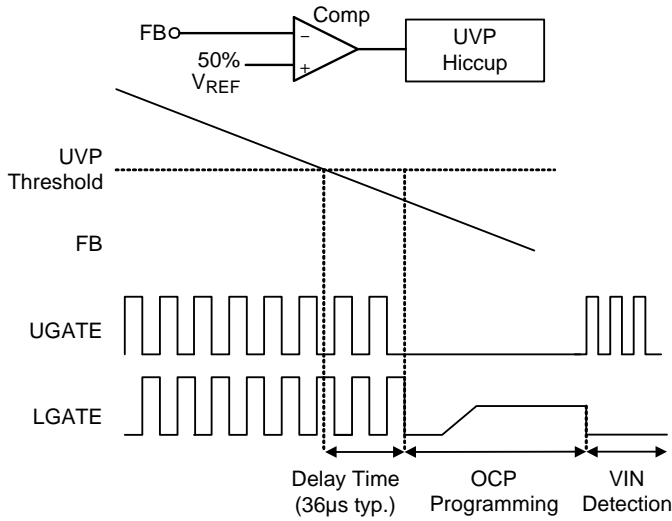
Figure 5. UVP Operation
