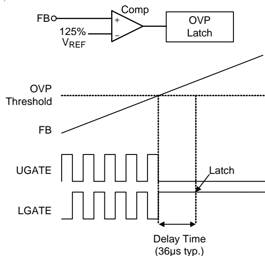
Figure 4. OVP Operation
