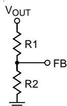
Figure 4. Setting V_{OUT} with a Resistive Voltage Divider
