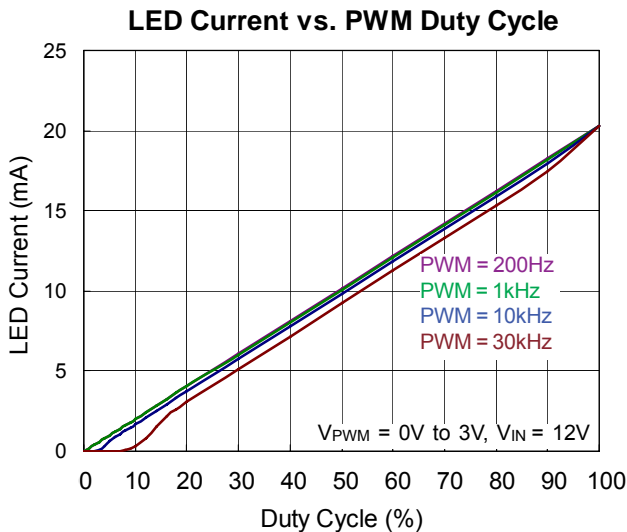
Figure 3. LED Current vs. PWM Dimming Duty Cycle
