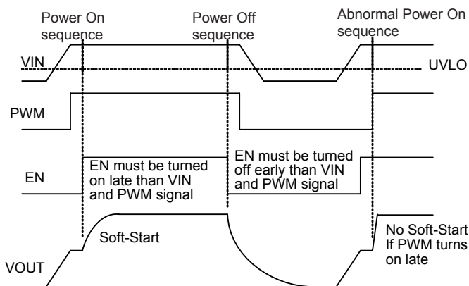
Figure 2. Power On Sequence Control by EN
