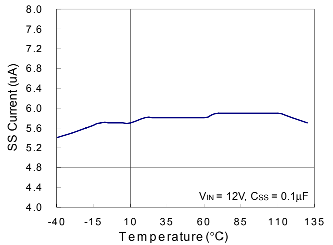
SS Current vs. Temperature
