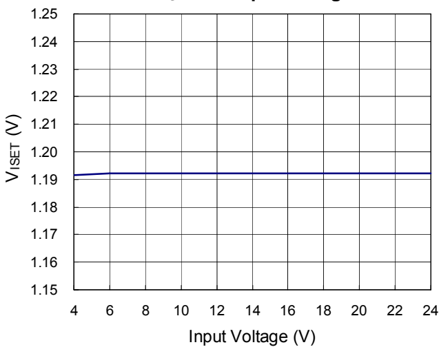
V SET vs. Input Voltage
