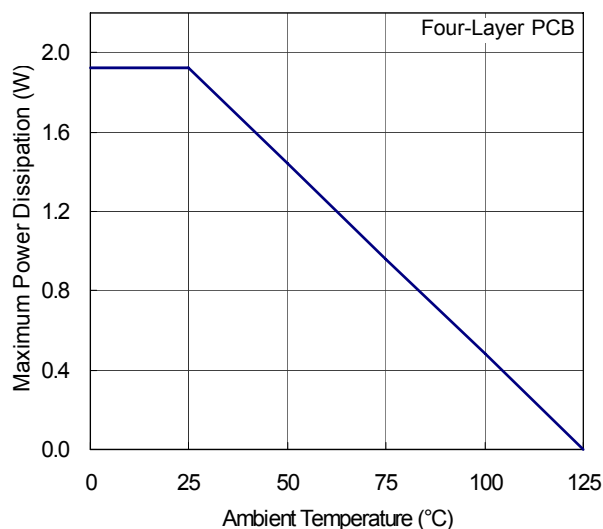
Figure 4. Derating Curve for RT8562B Package
