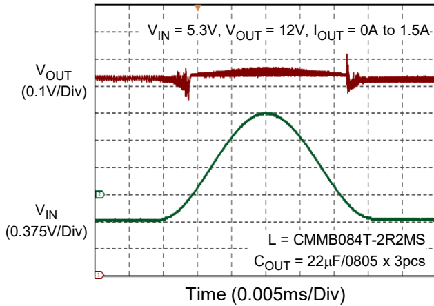
Stability
