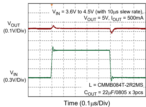
Line Transient
