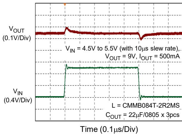
Line Transient
