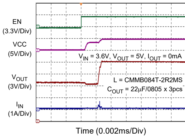
Power-On
