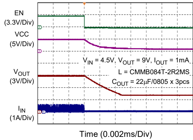
Power-Off
