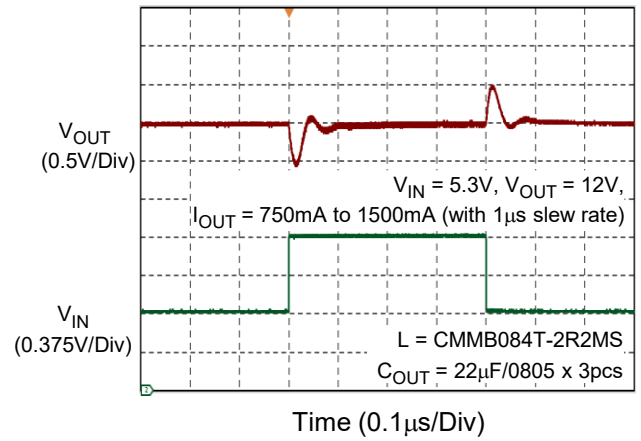
Load Transient
