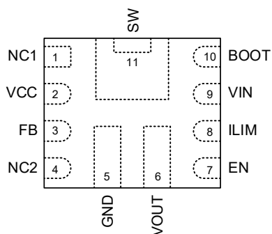
RT8581A/RT8581B
