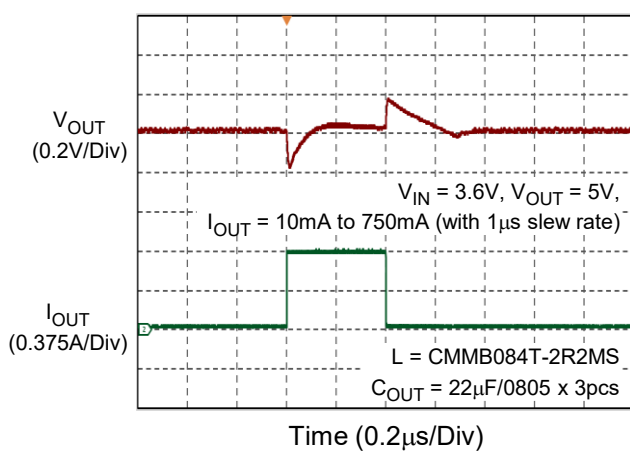
Load Transient
