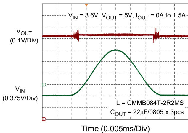
Stability
