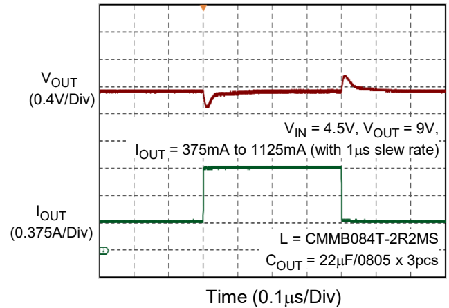
Load Transient
