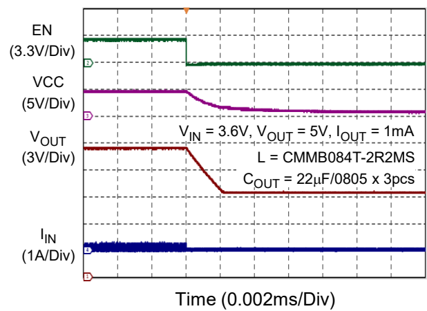
Power-Off
