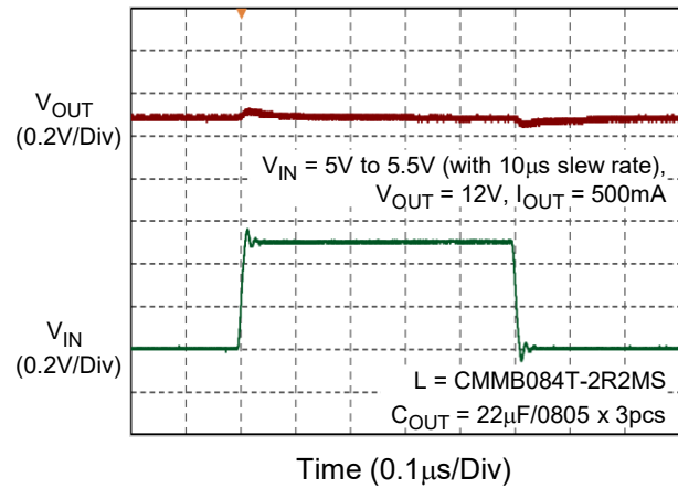
Line Transient
