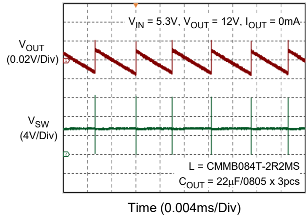
Output Ripple
