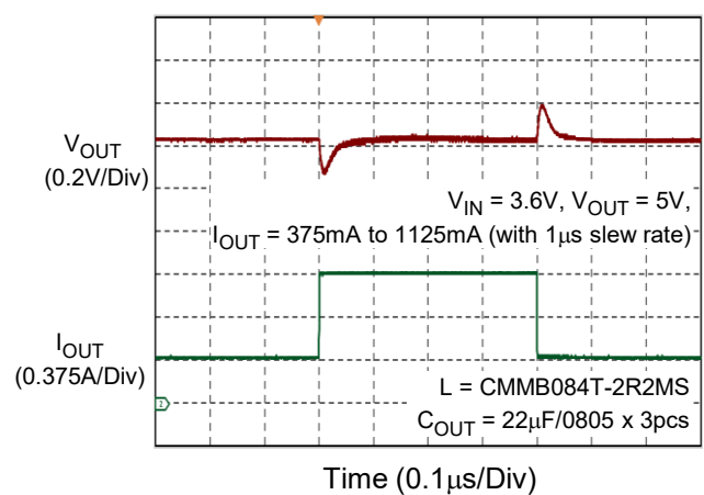
Load Transient
