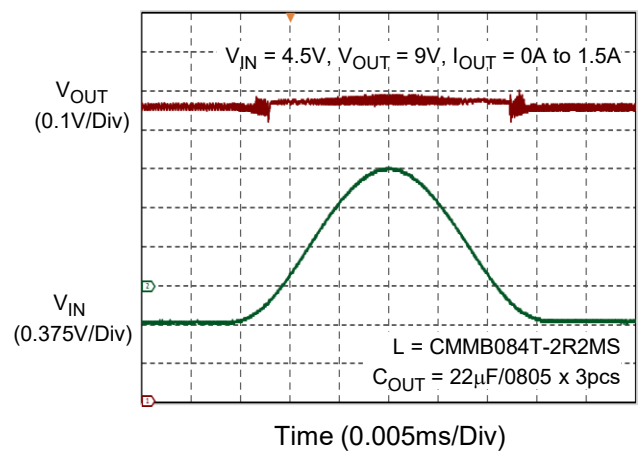
Stability
