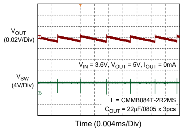
Output Ripple
