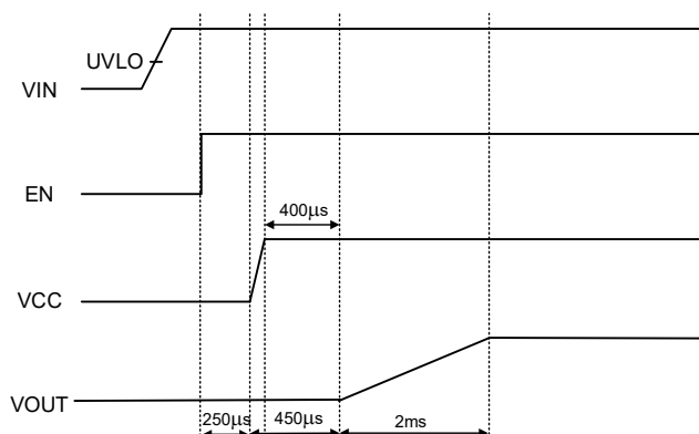
Figure 1. Soft-Start State
