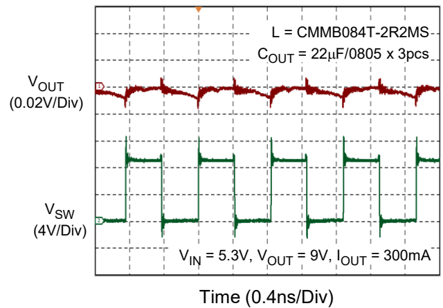
Output Ripple
