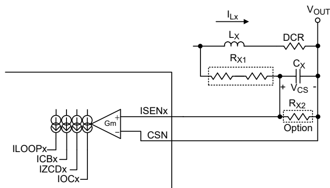
Figure 29. Inductor DCR Current Sensing Method
