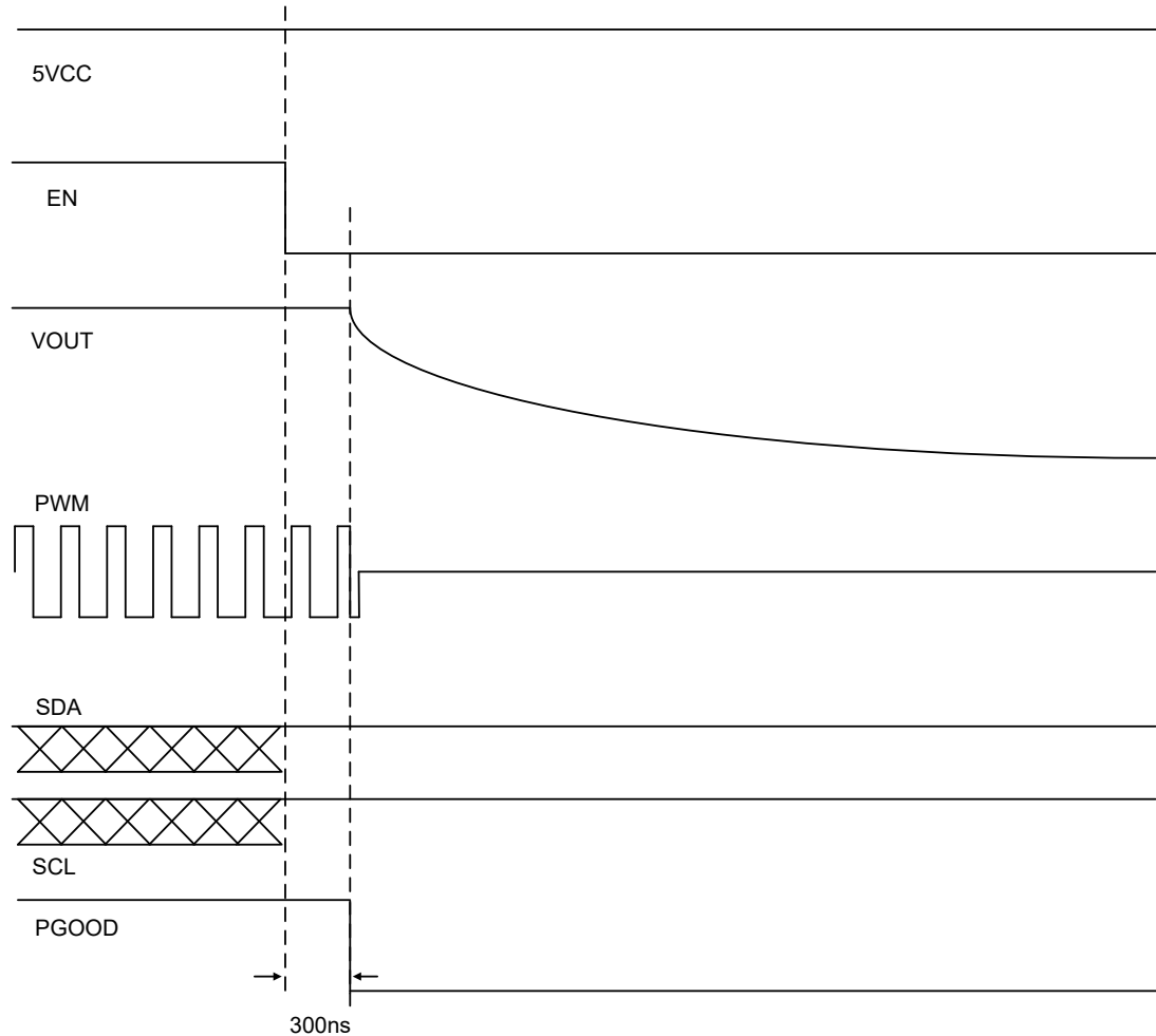
Figure 7. Power-Off Sequence of RT8848C by EN
