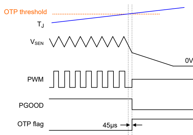
Figure 13. Typical OTP Protection Mechanism
