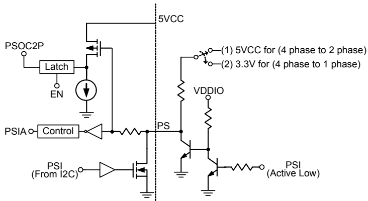
Figure 14. Power-Saving-Mode Circuit
