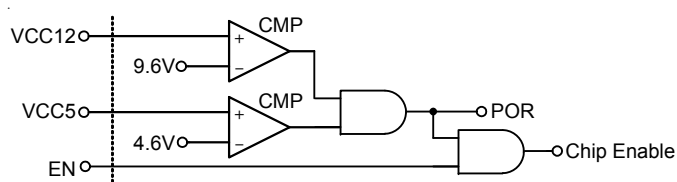
Figure 2. Circuit for Power Ready Detection
