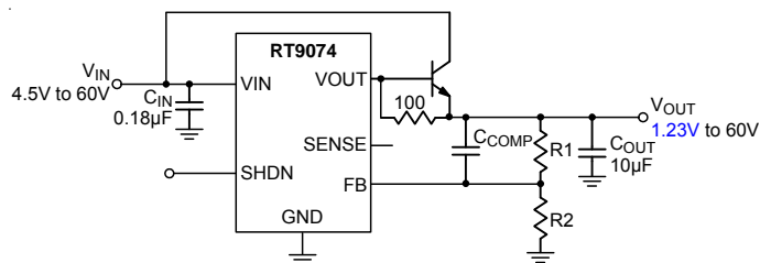
Figure 4. RT9074 External Transistor Application
