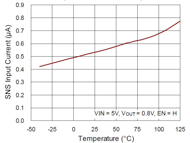
SNS Input Current vs. Temperature
