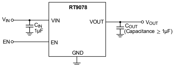
Figure 2. Application without Sense Function
