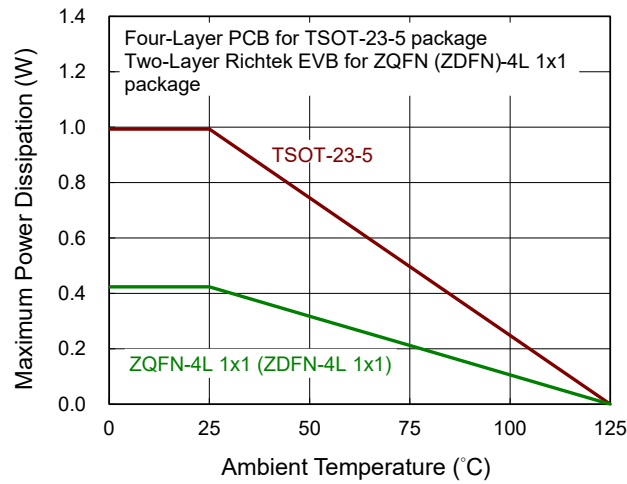
Figure 4. Derating Curves of Maximum Power Dissipation
