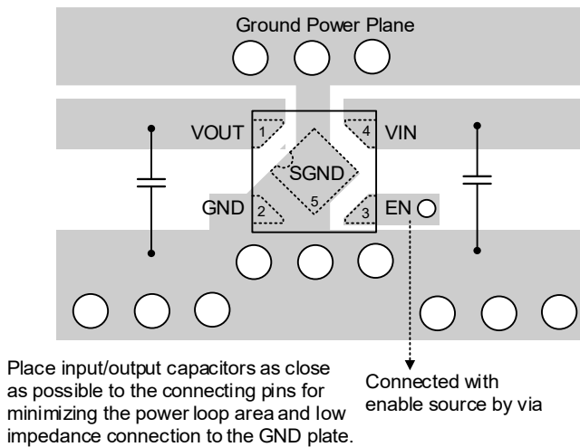
Figure 9. PCB Layout Guide for ZQFN-4L 1x1 Package
