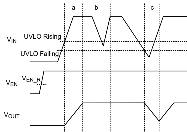
Figure 5. Undervoltage-Lockout Trigger Conditions and Output Variation
