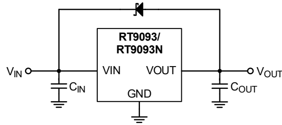
Figure 6. Application Circuit for Reverse Current Protection
