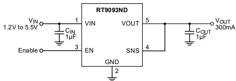
Figure 2. Configuration Circuit with SNS Pin for Fixed VOUT
