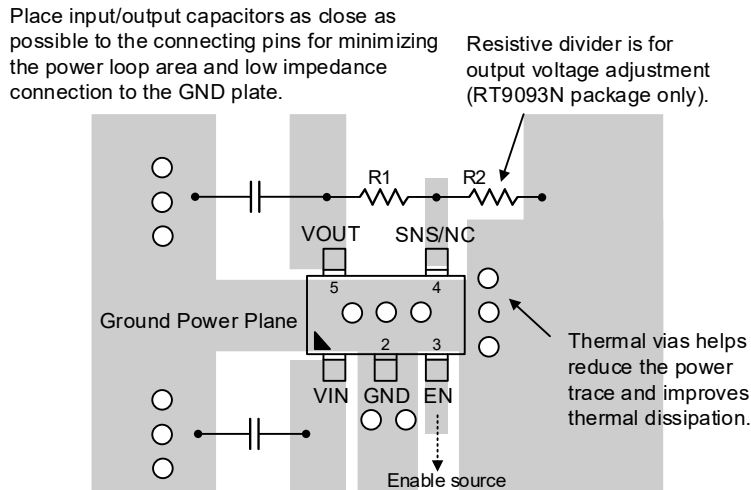
Figure 8. PCB Layout Guide for TSOT-23-5 Package
