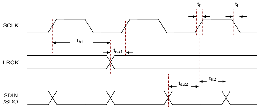
Figure 2. Timing Diagram of Slave Mode I 2 S Interface
