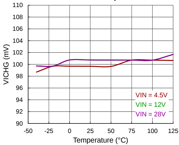
VICHG vs. Temperature
