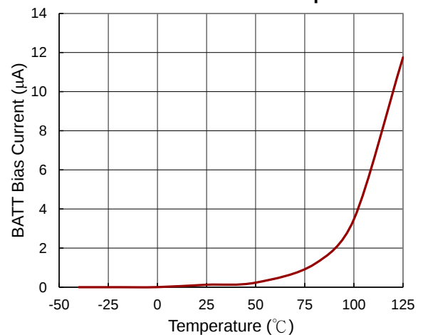
BATT Bias Current vs. Temperature
