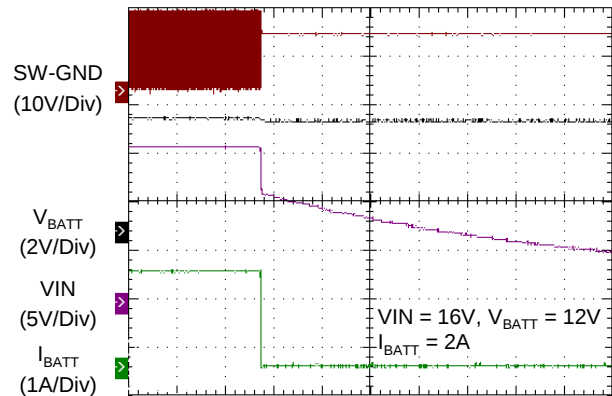
Adapter Remove
