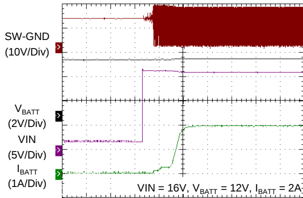
Adapter Insert
