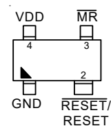
SC-82
