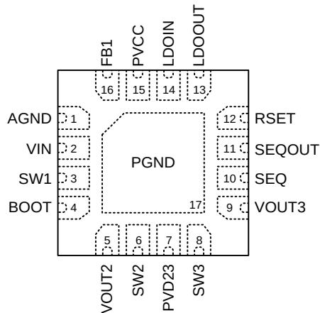
WETD-VQFN-16L 3x3 (RTQ2072A-QA)
