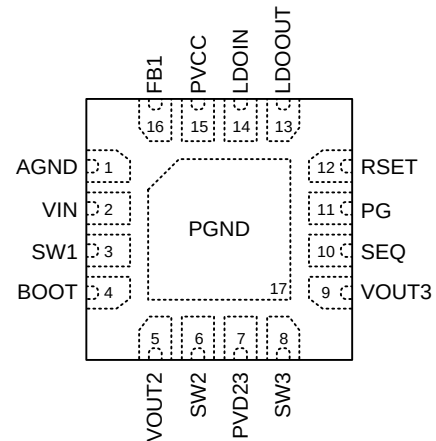
WETD-VQFN-16L 3x3 (RTQ2072B-QA)
