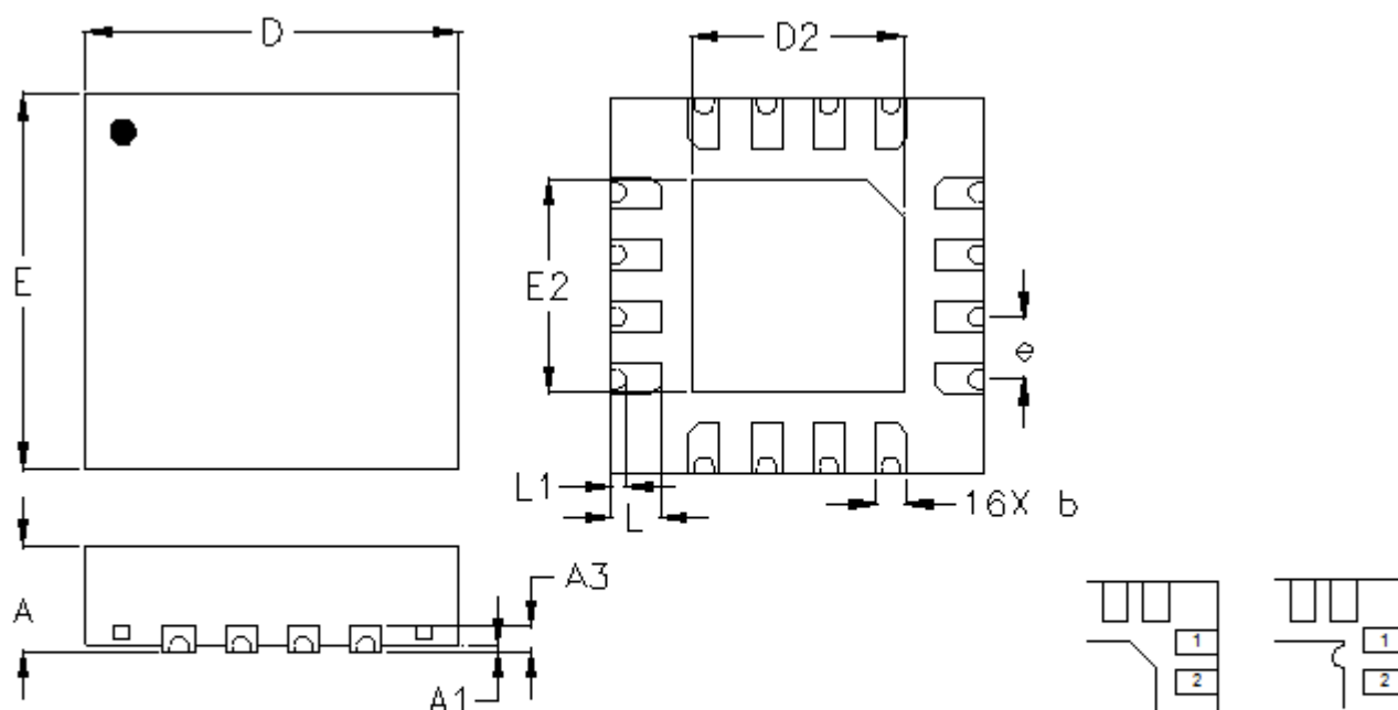
DETAIL A
